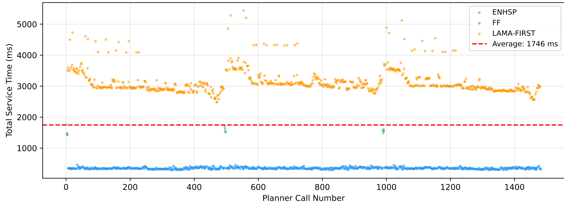
Planning Service Latency Per Call (With Replanning + LAMA-First)
